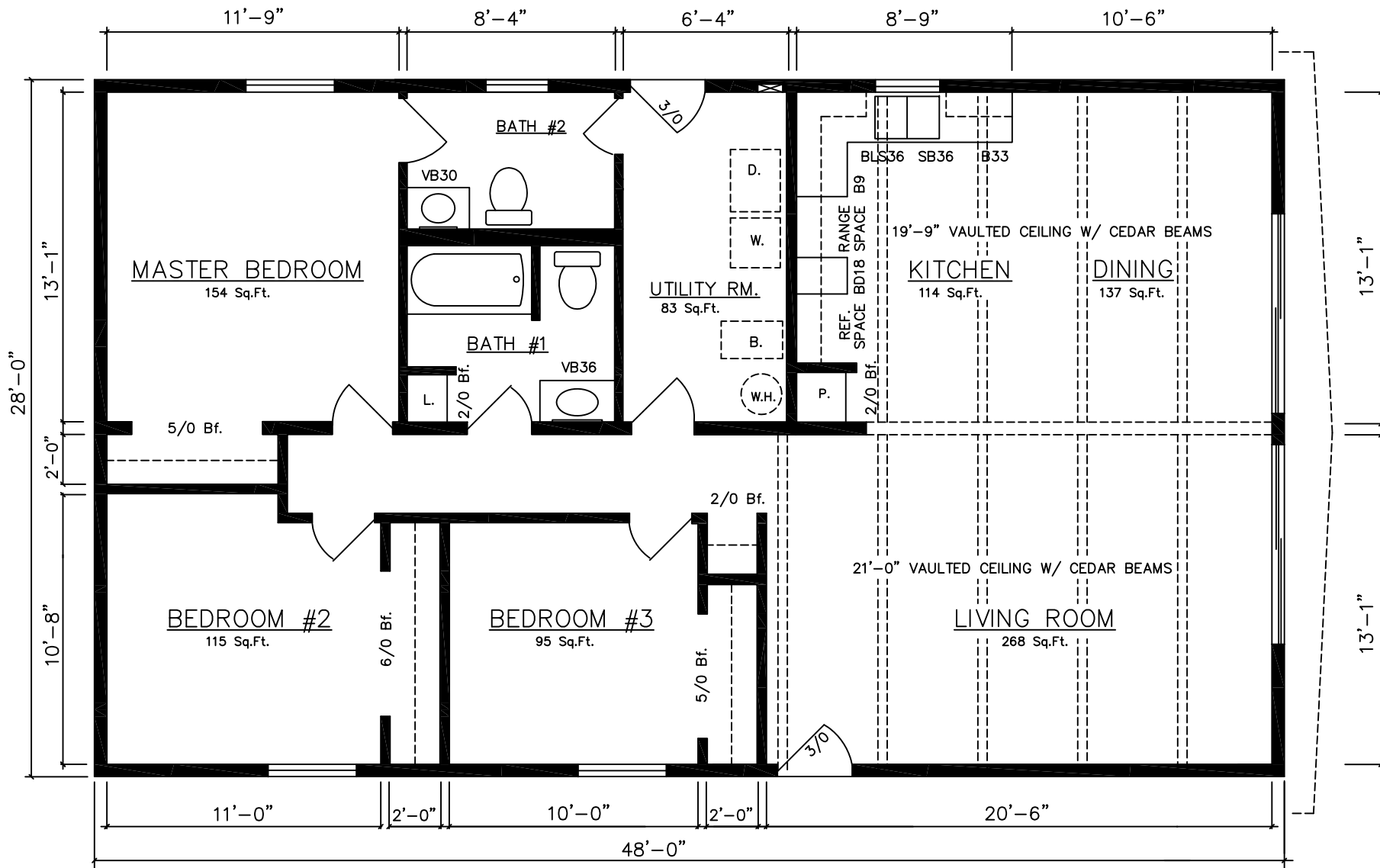
ALPINE 10702...(Crawlspace) 28'x48' (1,344 Sq.Ft.) 3 Bed, 1½ Bath
