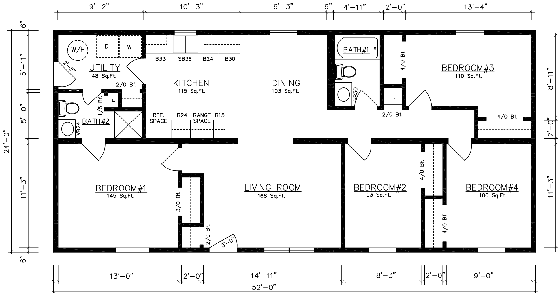
ALWOOD 14032...(Crawlspace) 24'x52' (1,248Sq.Ft.) 4 Bed, 2 Bath
