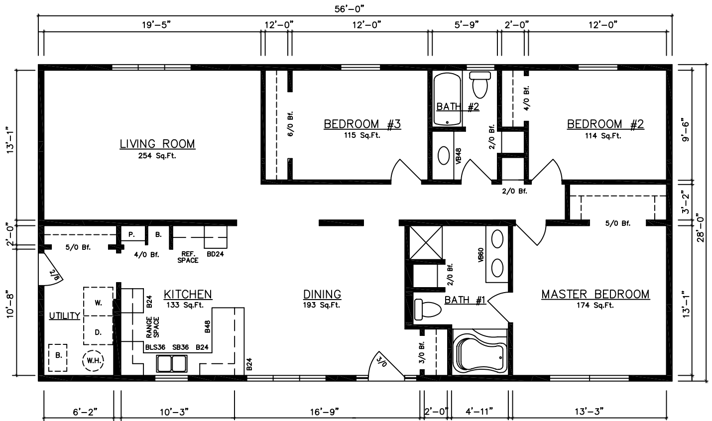
CHARLOTTE 10488...(Crawlspace) 28'x56' (1,568 Sq.Ft.) 3 Bed, 2 Bath
