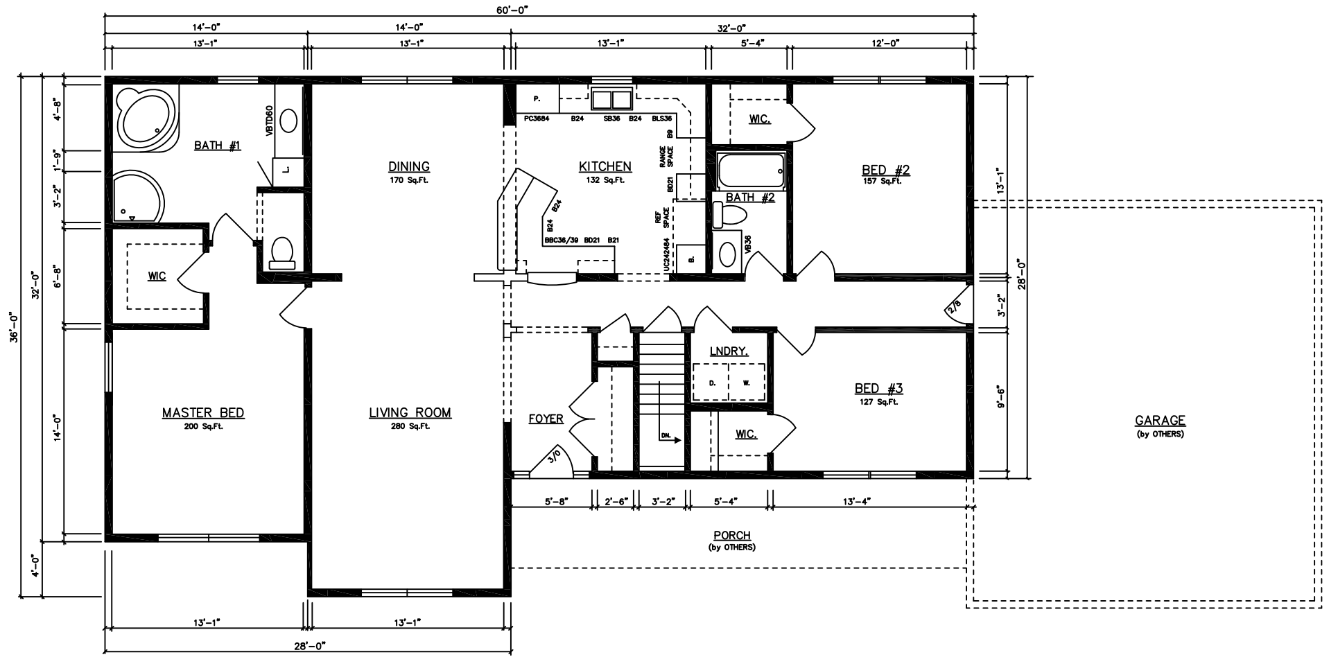
BASEMENT FLOOR PLAN (End Load Garage) ESSEX II...14106 (1848 Sq.Ft.)
