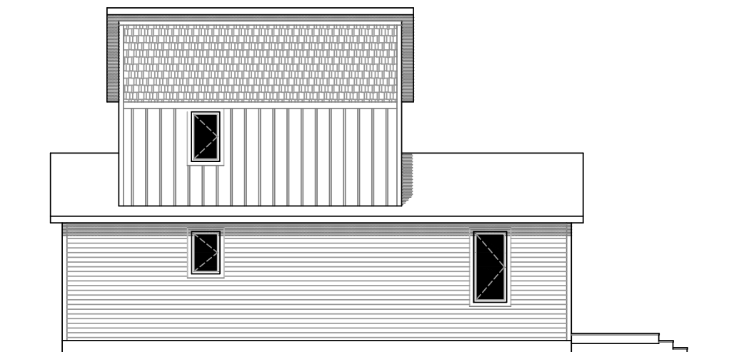
Left Elevation LEFT ELEVATION
