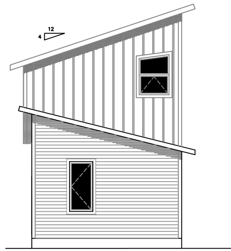
Rear Elevation REAR ELEVATION
