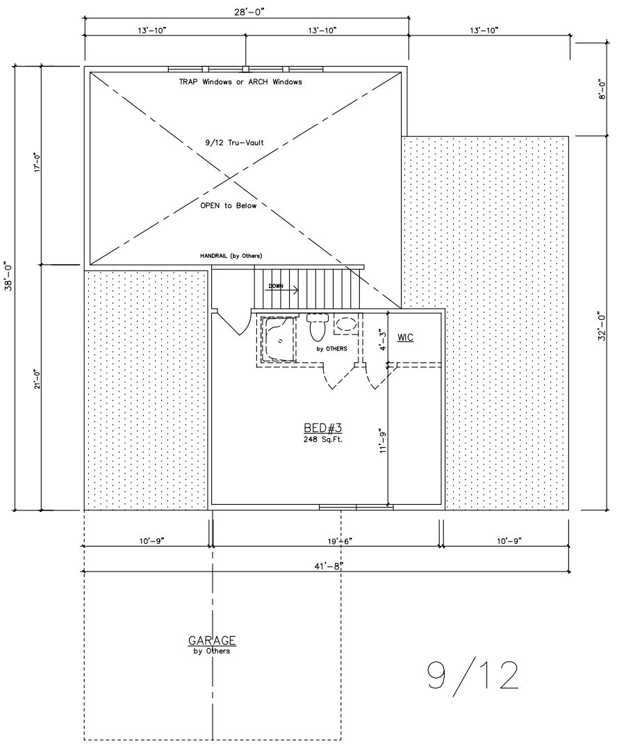
2nd Floor – Glen Arbor VI 358 Sq. Ft
