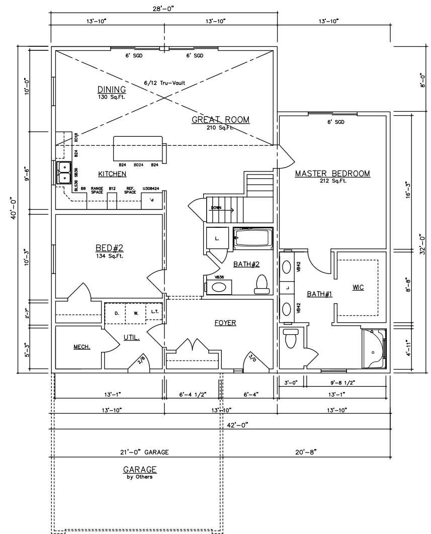
Glen Arbor III 14202 (Basement) 1,568 Sq. Ft.
