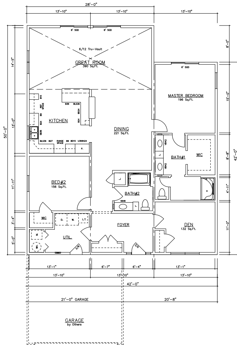
Glen Arbor 14156 (FLG - Crawl) 1,988 Sq. Ft.
