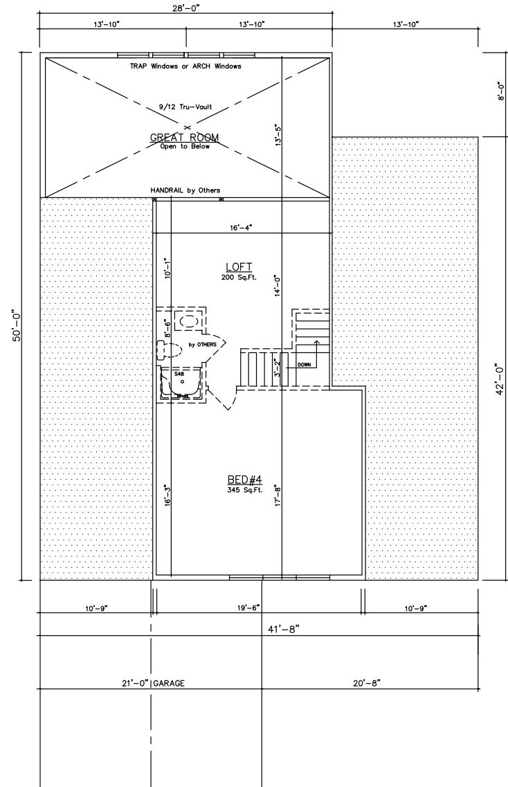
2nd Floor – Glen Arbor II 545 Sq. Ft
