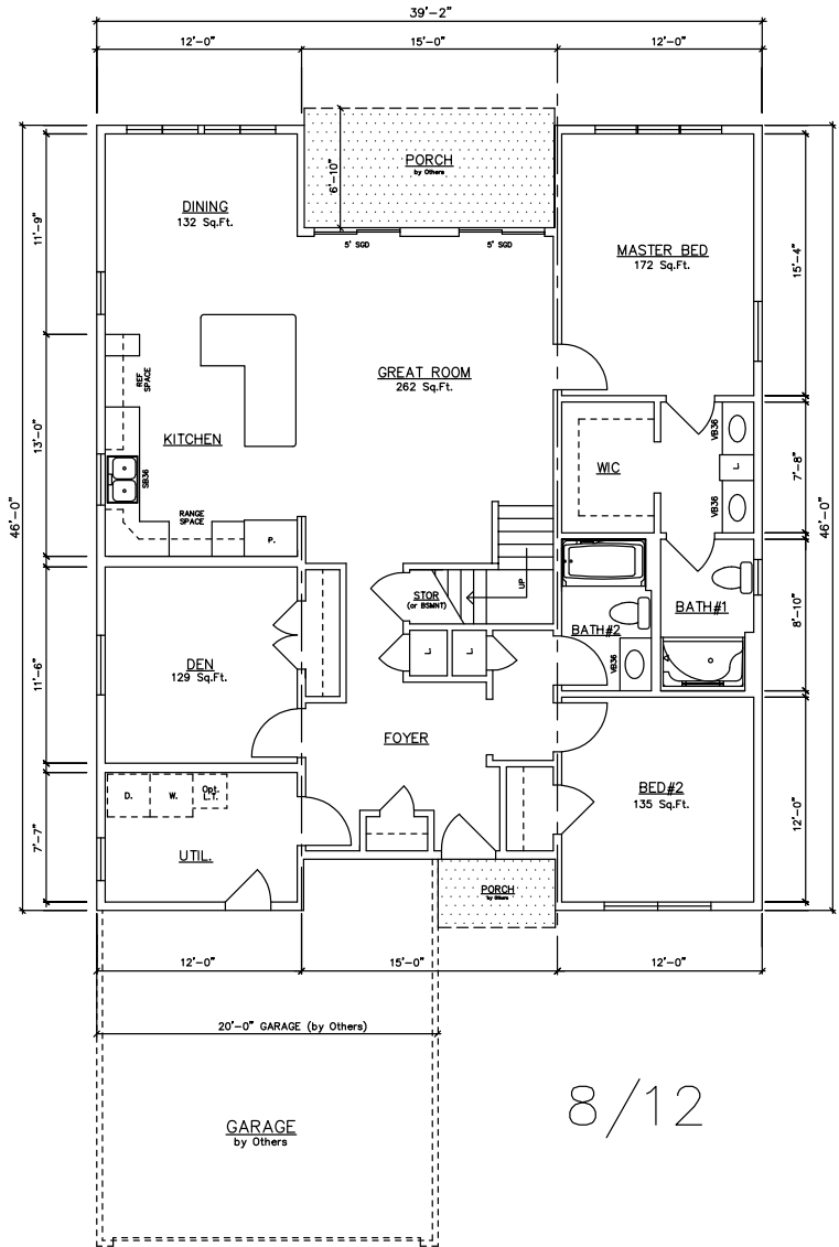
1st Floor – Grand Marais II 1,658 Sq. Ft. 14168 (Crawlspace) 14170 (Basement)
