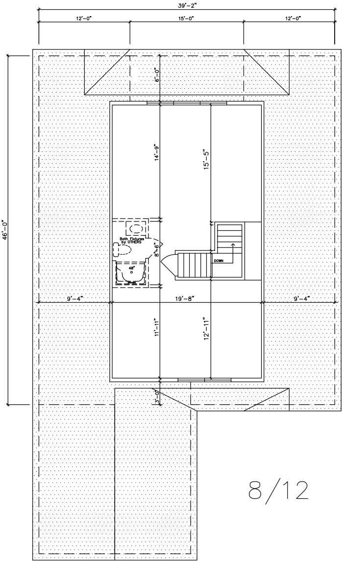
2nd Floor – Grand Marais II 730 Sq. Ft
