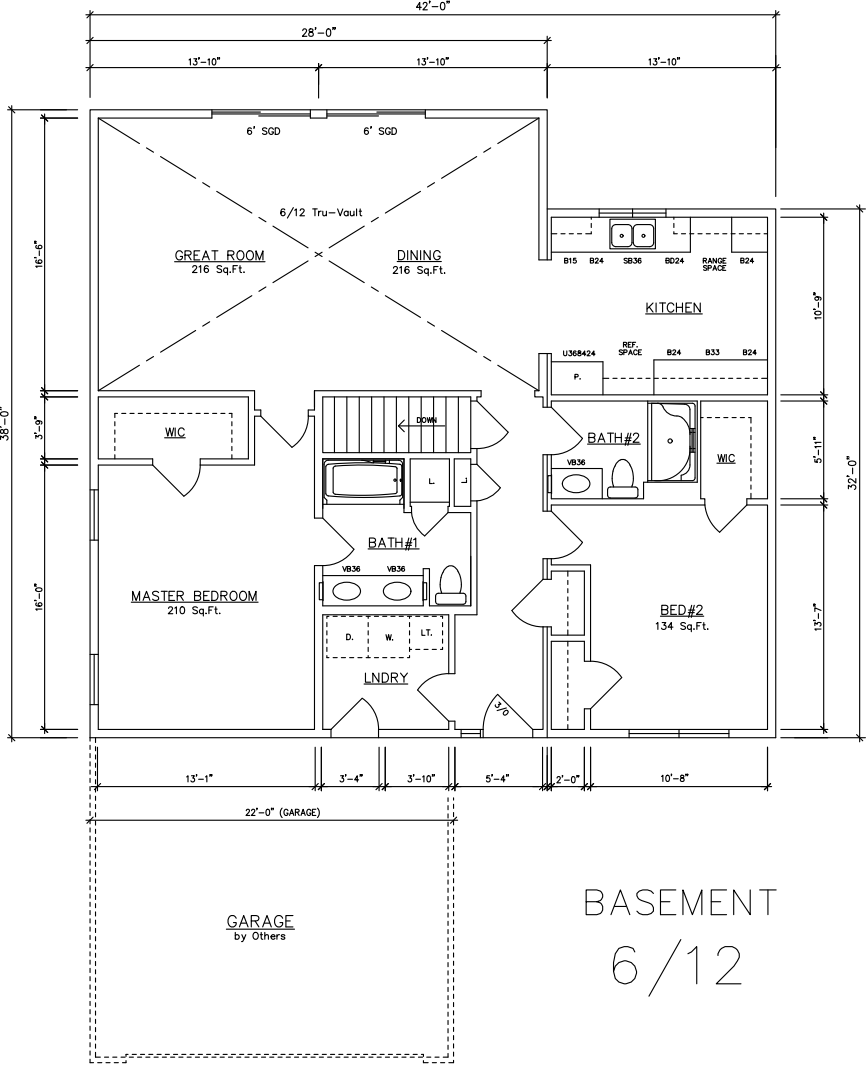
Glen Arbor V 14210 (Basement) 1,512 Sq. Ft.
