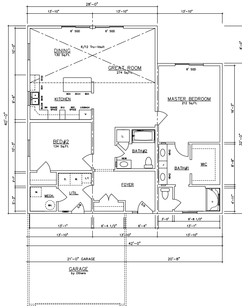
Glen Arbor III 14200 (Crawl) 1,568 Sq. Ft.
