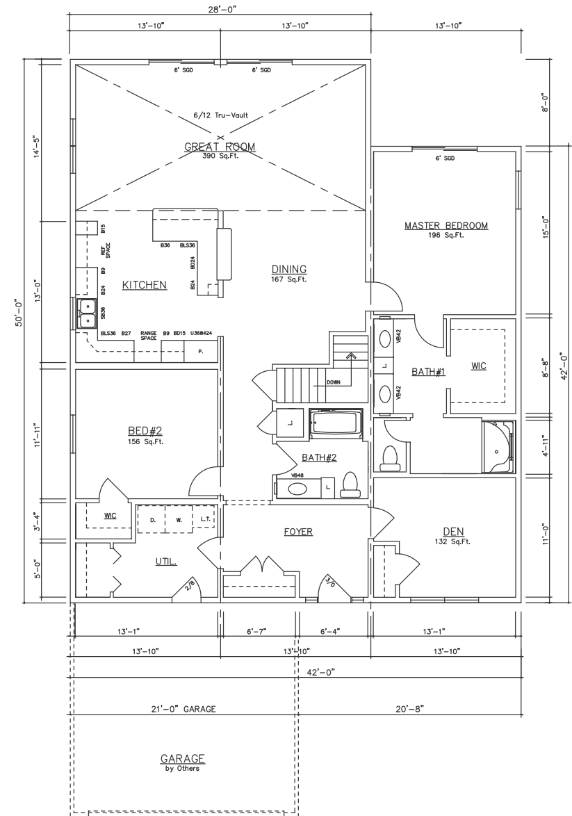
Glen Arbor 14158 (FLG - Basement) 1,988 Sq. Ft.
