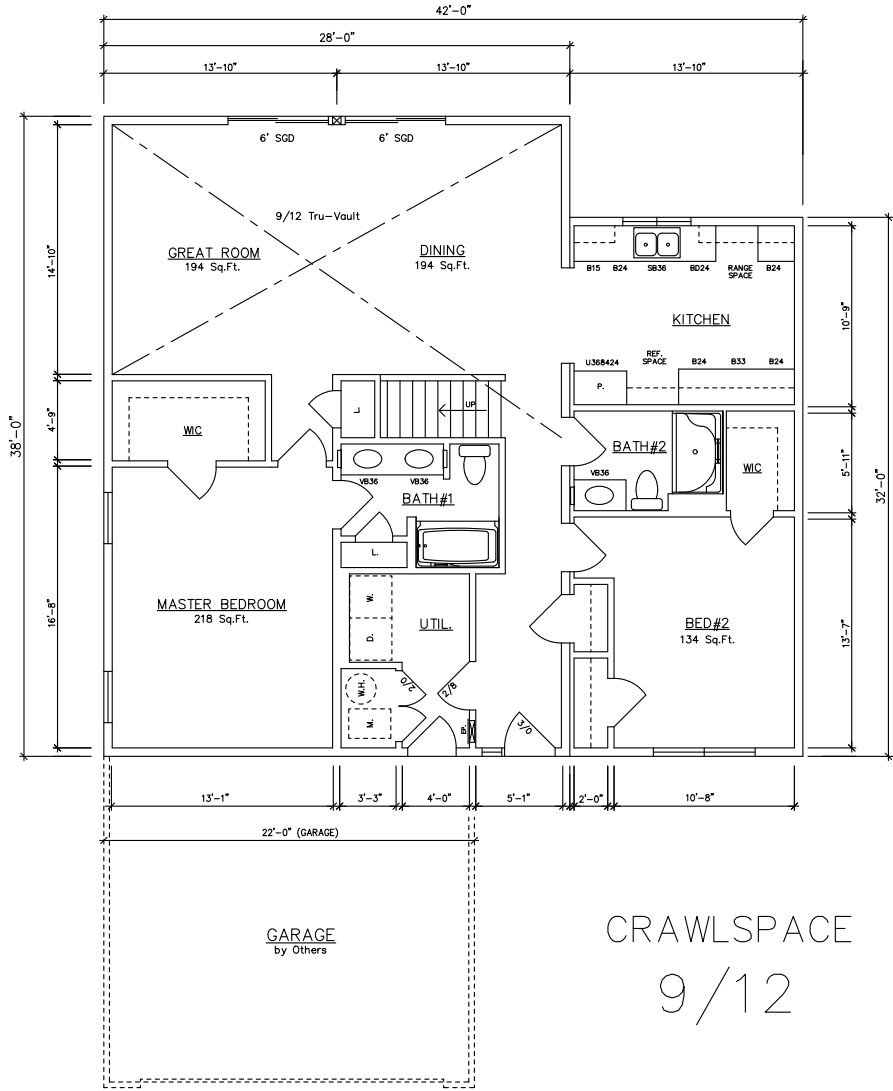
1st Floor – Glen Arbor VI 1,512 Sq. Ft. 14212 (Crawlspace)
