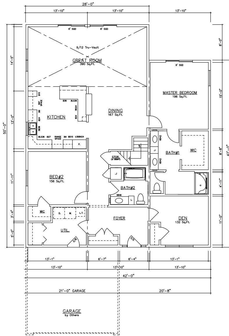
1st Floor – Glen Arbor II 1,988 Sq. Ft. 14160 (Crawlspace) 14162 (Basement)
