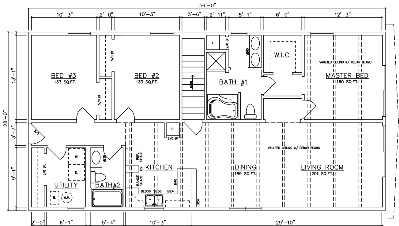
Alpine 10752 (Basement) 1,568 sq. ft.
