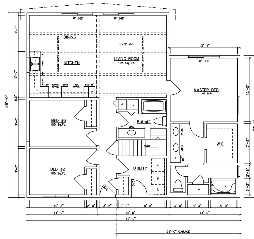
Alpine III 14226 (Basement)
