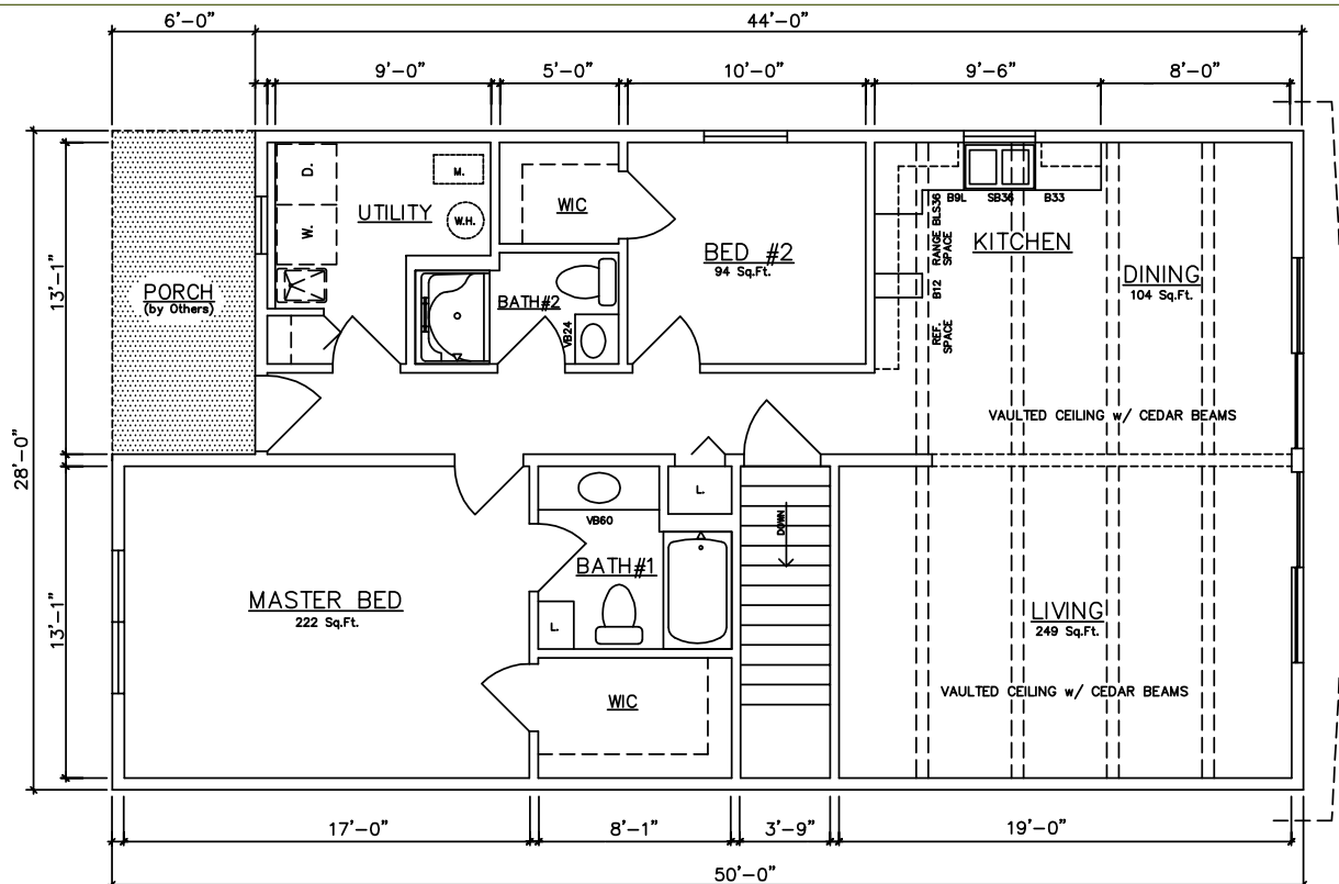
Alpine 10614 (Basement) 1,316 sq. ft.
