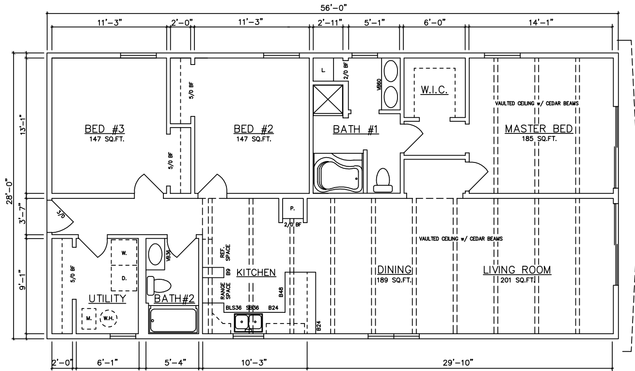
Alpine 10750 (Crawlspace) 1,568 sq. ft.
