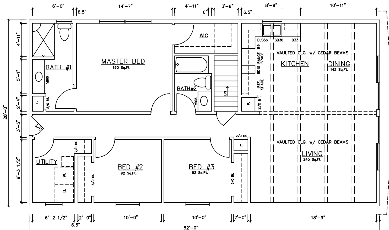
Alpine 10726 (Basement) 1,456 sq. ft. End Load Garage
