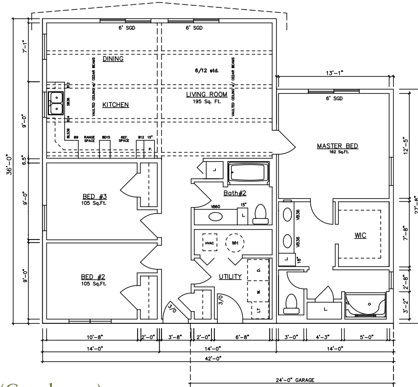
Alpine III 14224 (Crawlspace)
