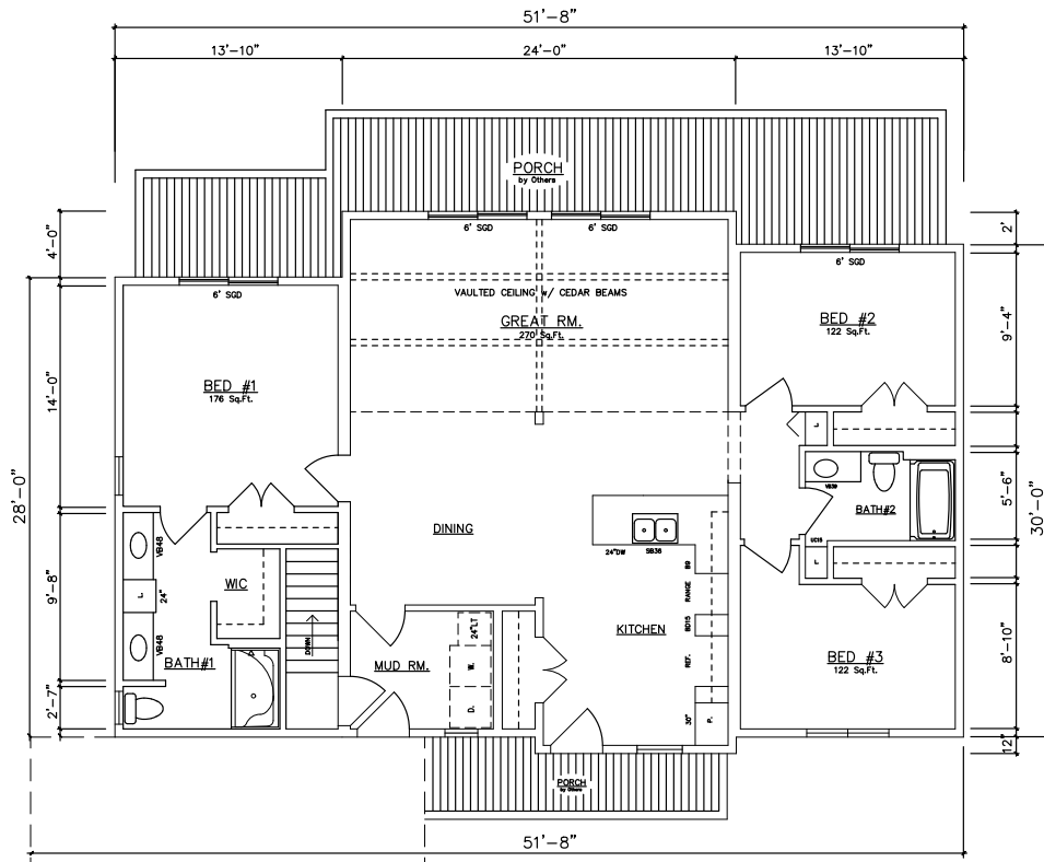
Alpine IV 10776 (Basement)
