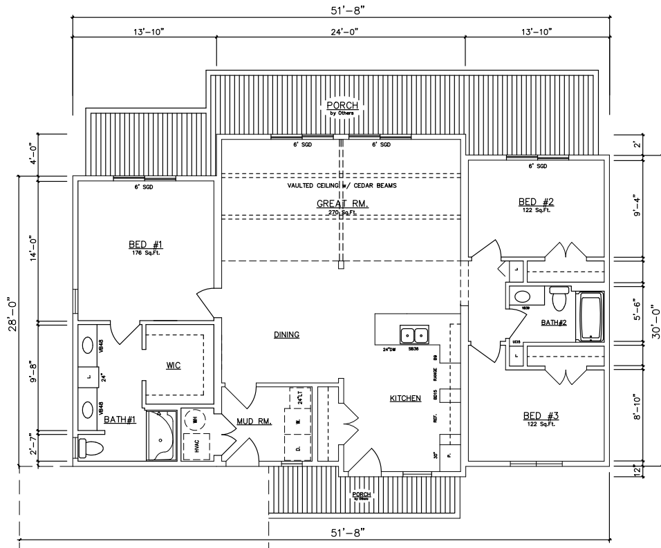
Alpine IV 10774 (Crawlspace)
