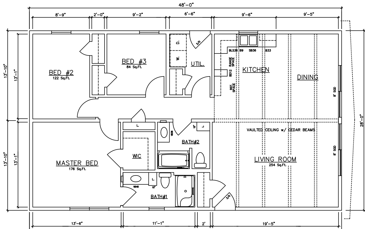
Alpine 10716 (Crawlspace) 1,344 sq. ft.
