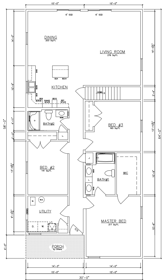
30' WIDE OPTION
