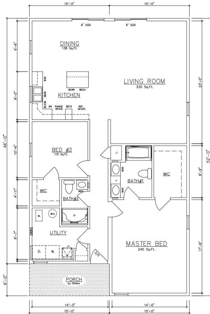
30' WIDE OPTION
