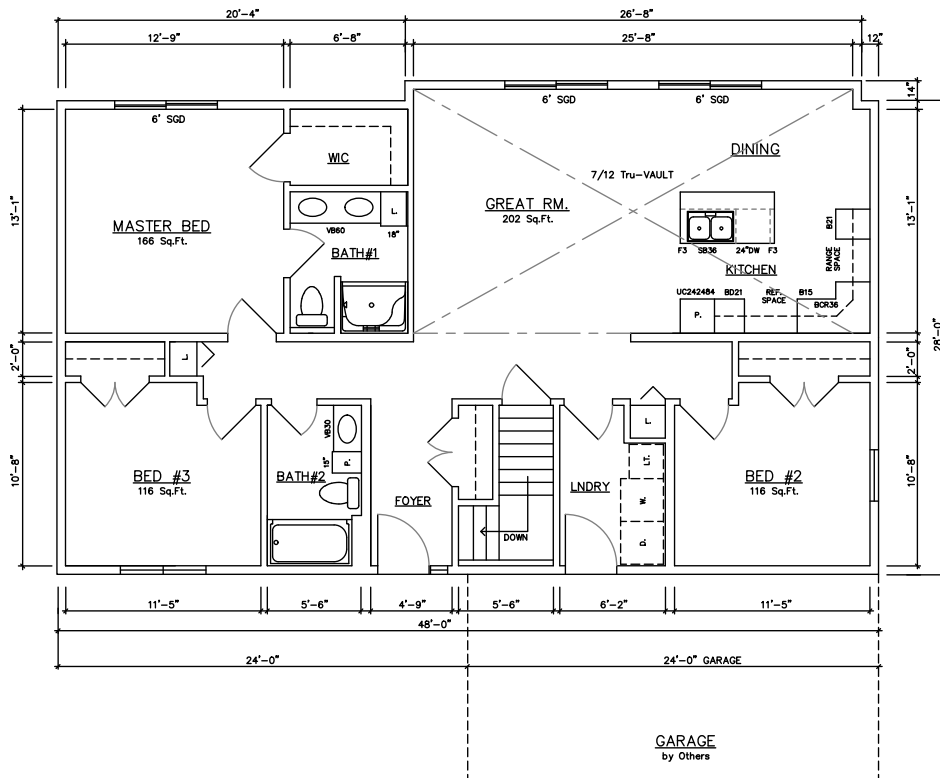
Indian River 10568 (Basement) 1,374 sq. ft.
