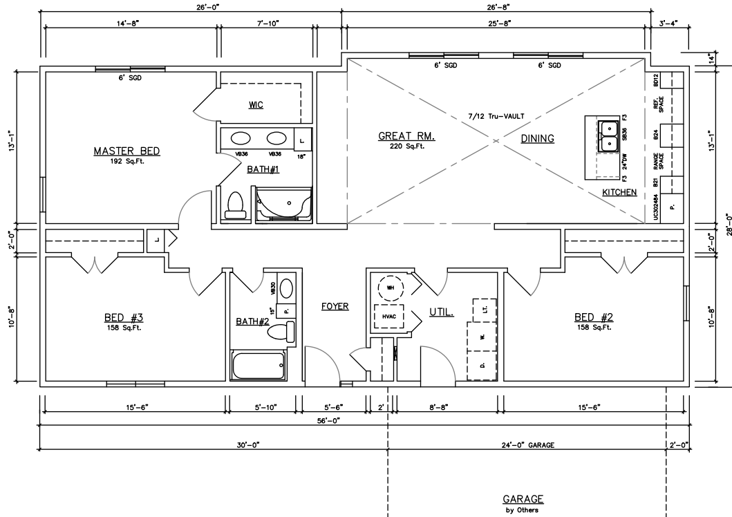
Indian River 10574 (Crawlspace) 1,598 sq. ft.
