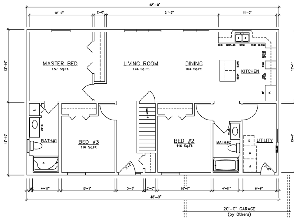
Lakeview 10580 (Basement) 1,344 sq. ft.
