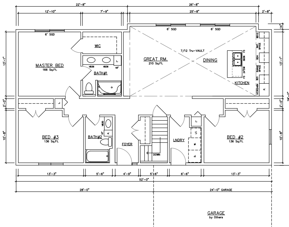
Indian River 10572 (Basement) 1,486 sq. ft.
