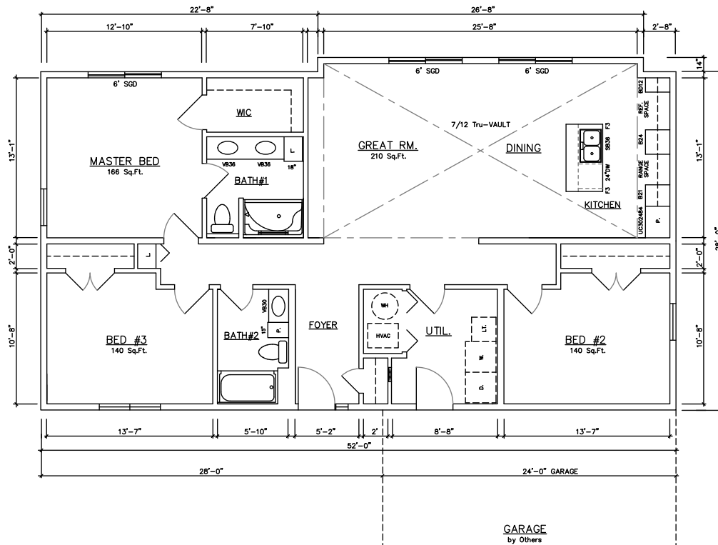
Indian River 10570 (Crawlspace) 1,486 sq. ft.
