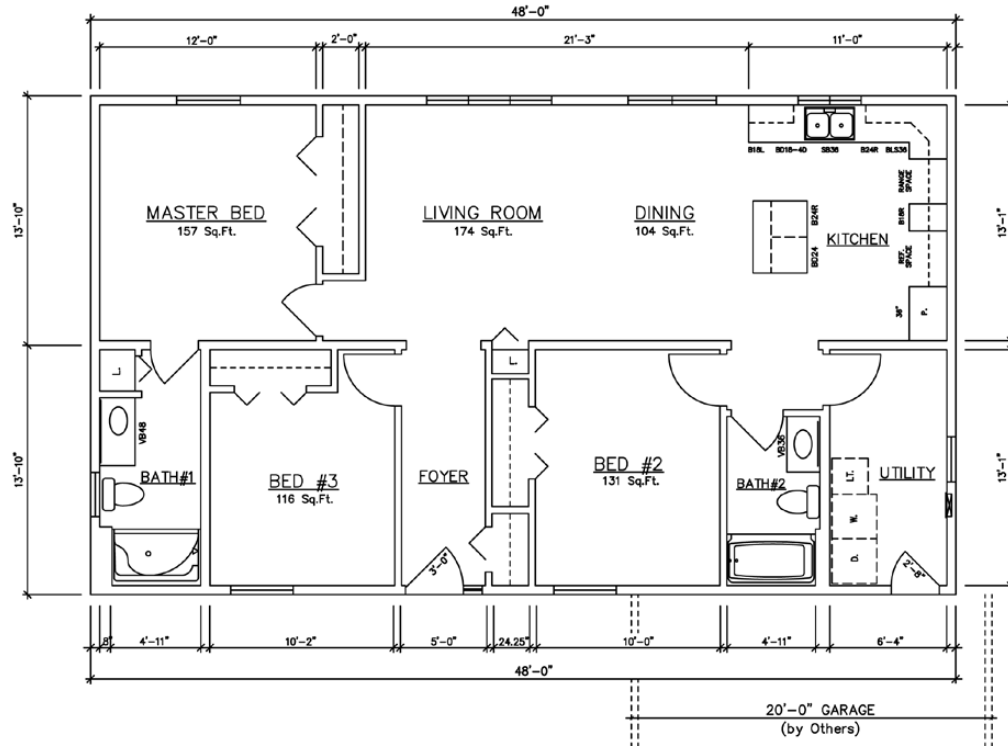
Lakeview 10578 (Crawlspace) 1,344 sq. ft.
