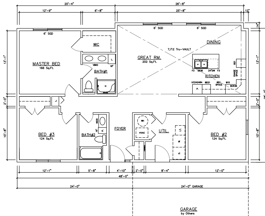
Indian River 10566 (Crawlspace) 1,374 sq. ft.
